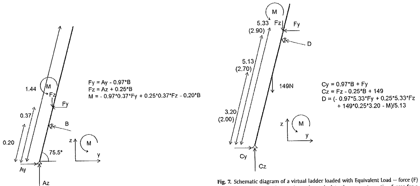
Fig. 6. Schematic diagram of the ladder physical model support and loading conditions, and calculations for Equivalent Load, i.e., force (F) and moment (M). The coordinate system on the right indicates the positive directions for forces and moment. Ay – horizontal reaction force at the base of the ladder section. Az – vertical reaction force at the base of the ladder section. B – normal reaction force at the edge of the roof structure. Fy – equivalent horizontal force at the rung next to roof edge. Fz – equivalent vertical force at the rung next to roof edge. M – equivalent moment associated with Fy and Fz.
